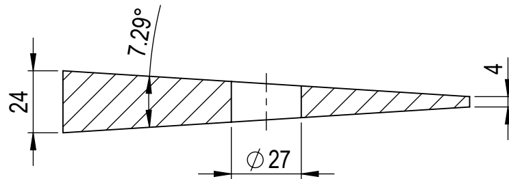
SECTION BC-BC
